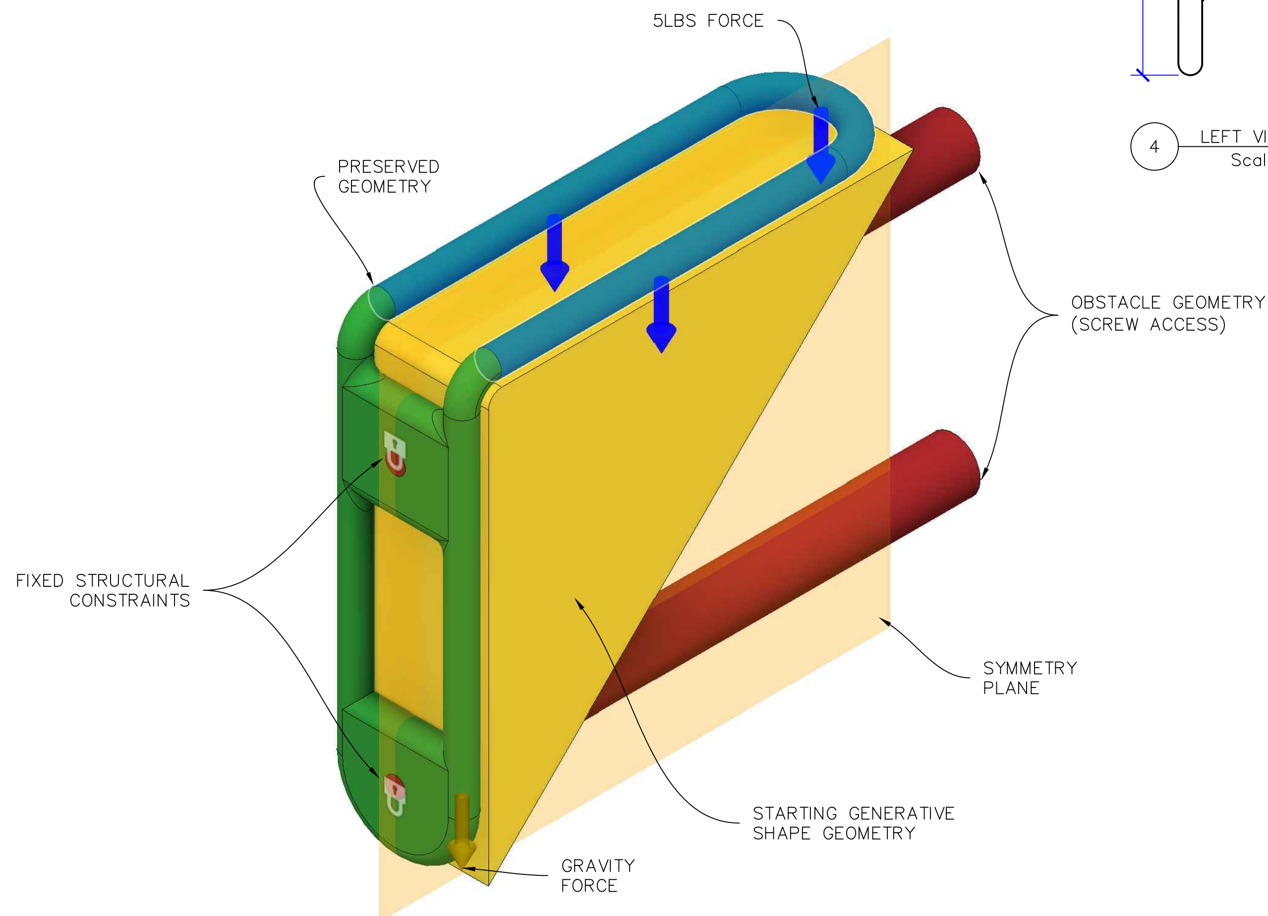
2 GENERATIVE DESIGN DETAILS Scale: NTS
